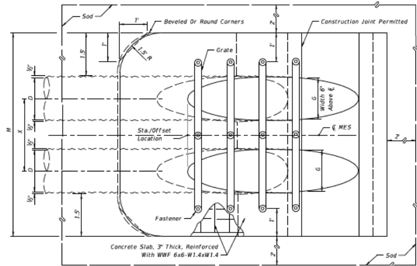
TOP VIEW-MULTIPLE PIPE
