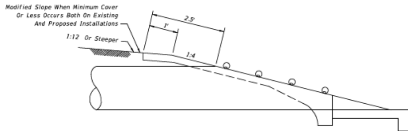
PERMISSIBLE PAVEMENT MODIFICATION
