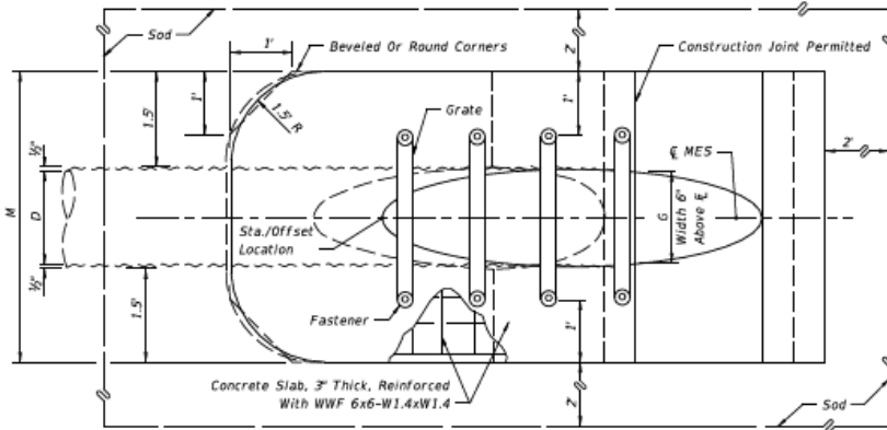
TOP VIEW-SINGLE PIPE
