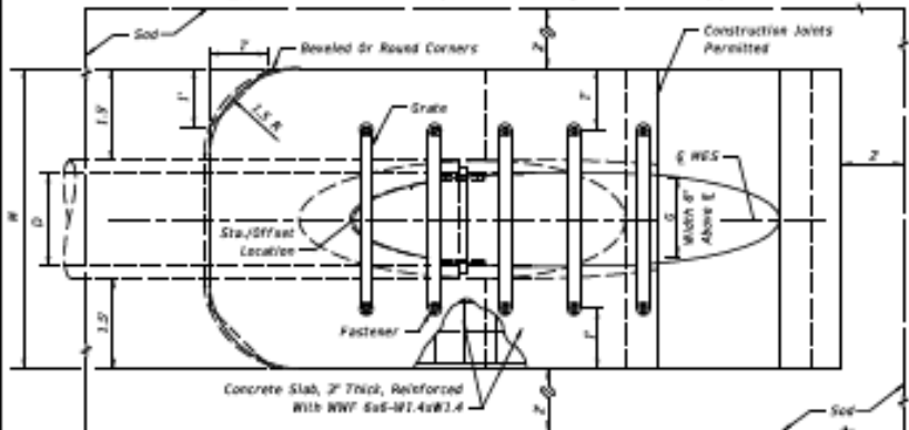
TOP VIEW-SINGLE PIPE
