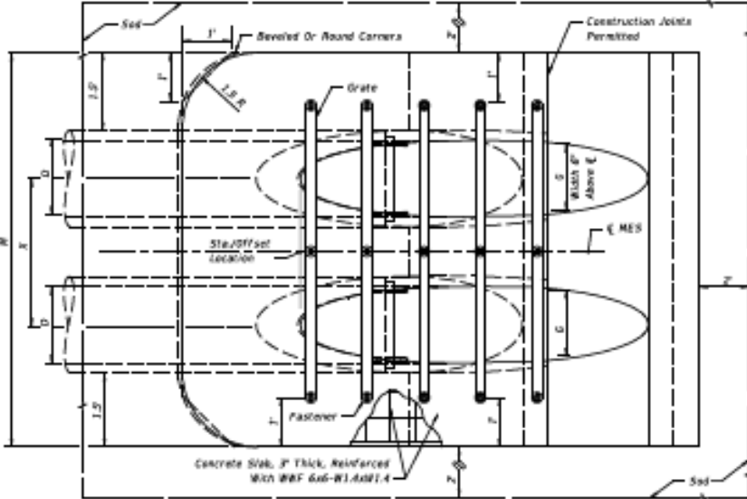
TOP VIEW-MULTIPLE PIPE
