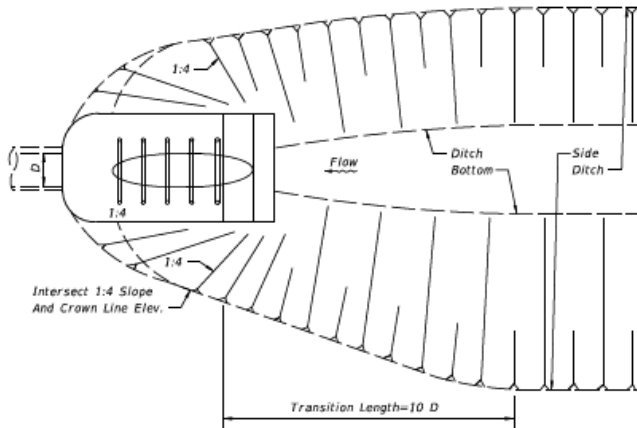
PLAN DITCH TRANSITION
